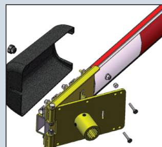
HyProtect breakaway arm bracket assembly.
